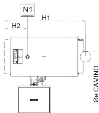
VISTA IN PIANTA plan view
